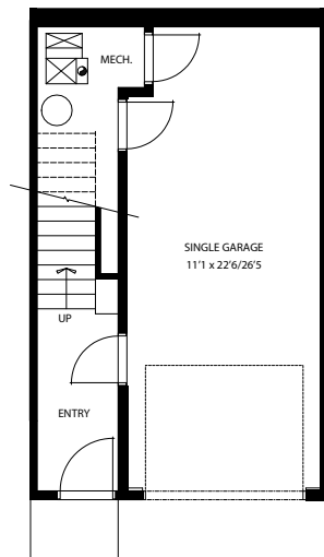
Garage Level 59 sq. ft.
